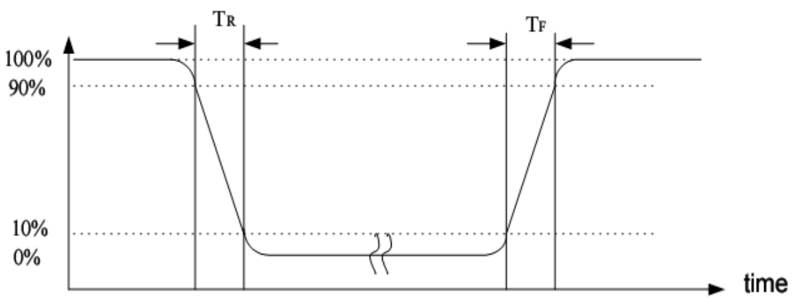
Figure 5. Definition of response time: T_r + T_f
