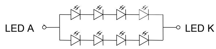
LED CIRCUIT
